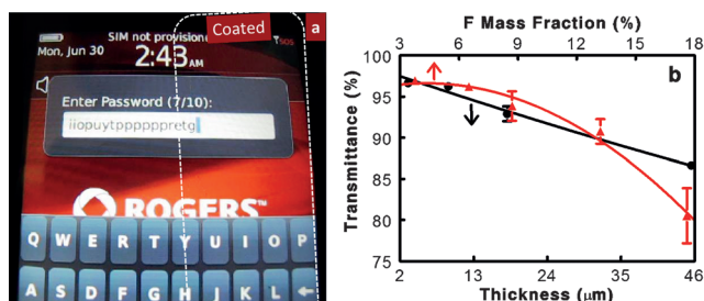
Figure 2. a) Photograph of a smartphone that was coated in the region enclosed by the dashed box. The P3-modified coating was 15\ \mu\text{m} thick and had a fluorine content of 7.2 wt %. b) Transmittance variation at 500 nm for P3-modified coatings as a function of film thickness at 6.6 wt % fluorine (black curve) and as a function of the fluorine mass fraction at a fixed thickness of (15 \pm 2)\ \mu\text{m} (red curve).
